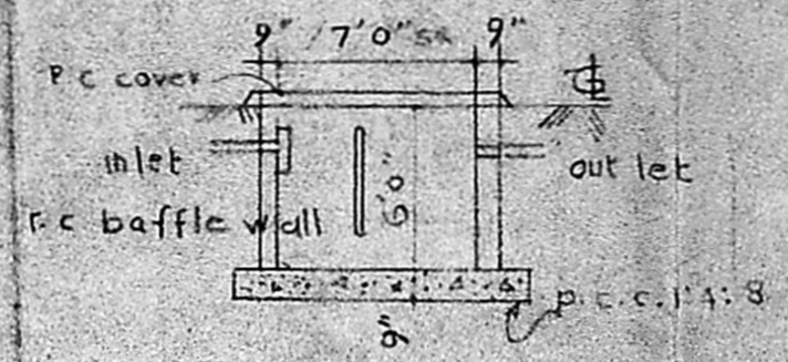
septic tank
